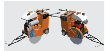
POSSIBILITY TO MOUNT THE BLADE ON THE LEFT OR RIGHT SIDE
